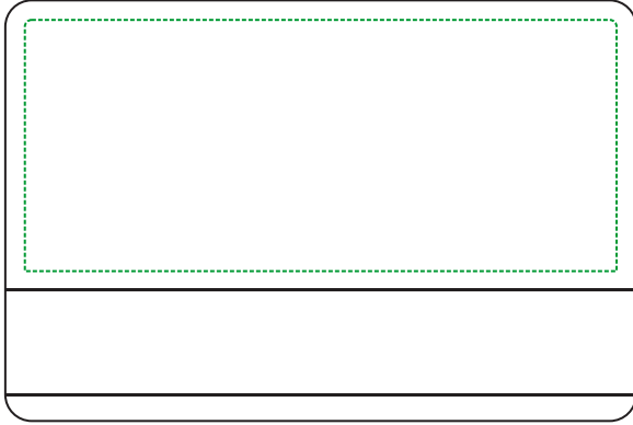
2"x 3" 60Mil Plastic Badge - 1/8 Radius Corners - 1/2" Strip
